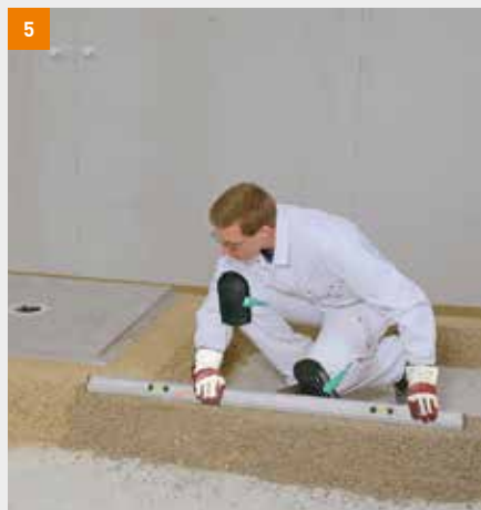
5 The second levelling edge is then laid out and aligned
