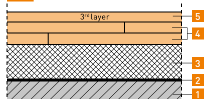
fermacell Flooring Element with additional insulation and 3 rd layer, e.g. 2 E 22 with 3 rd layer on EPS hard foam insulation
