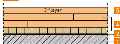
fermacell flooring element with additional 3 rd layer, without additional insulation, e.g. 2 E 31 Levelling only with fermacell Self-Levelling Compound, Bonded Levelling Compound, Honeycomb Insulation System
