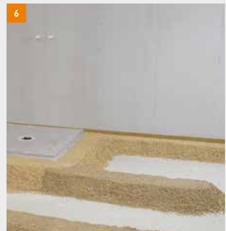
6 Wait until the levelling edges are dry (approx. 20 minutes)
