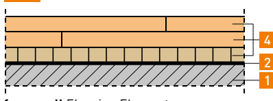
fermacell Flooring Element without additional insulation, e.g. 2 E 31
